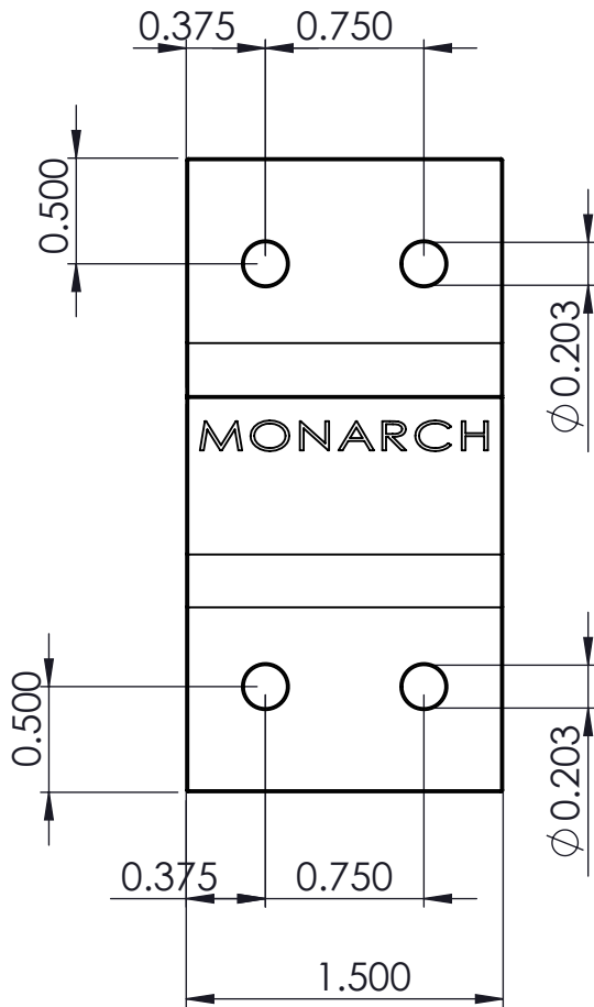
Full Scale Assembly (Two identical parts)
