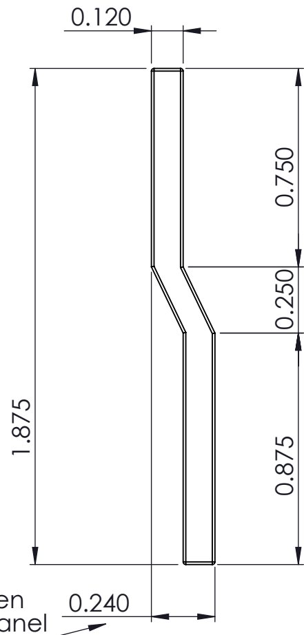
Vertical Section of one part
