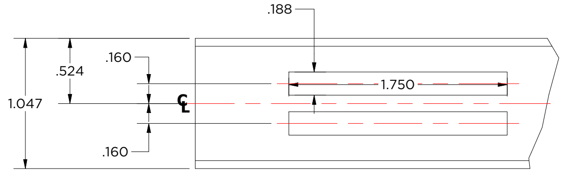
DETAIL P SCALE 1.33 : 1
